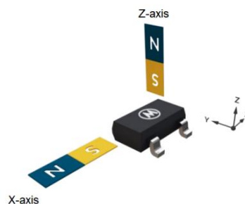
Fig 4A, 3D (X/Z-Axis) Magnetic Operation of AS11910D
