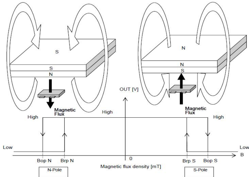
Fig 4B, X/Z-Axis Magnetic Operation Characteristic of AS1191OD
