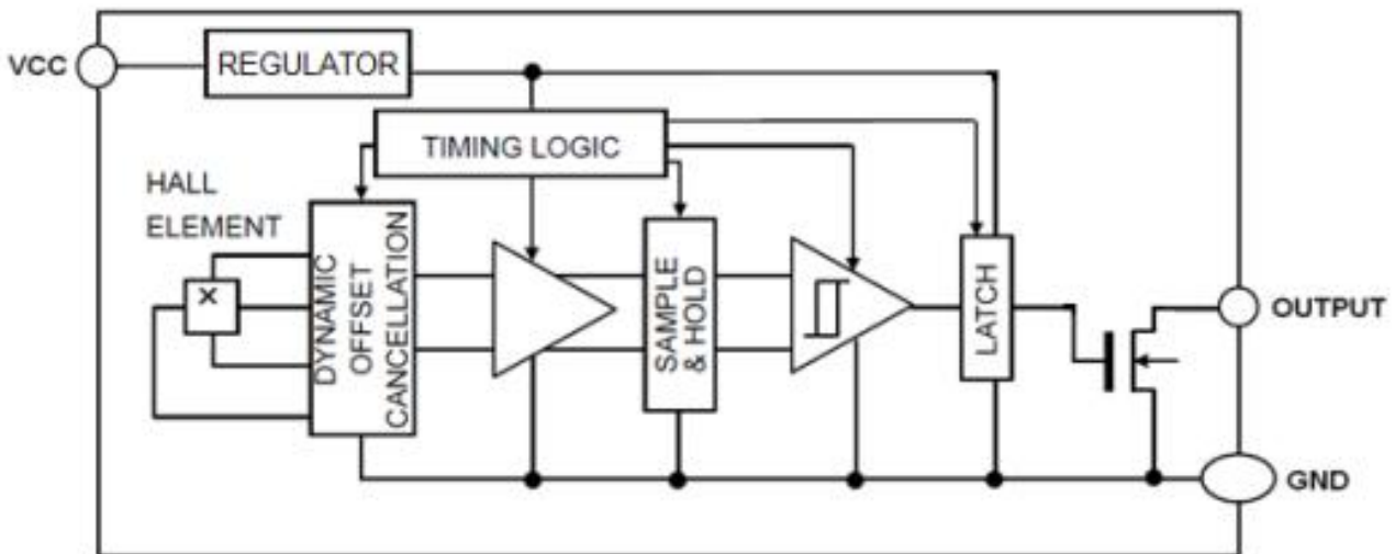
Figure 3, Block Diagram of AS1191OD
