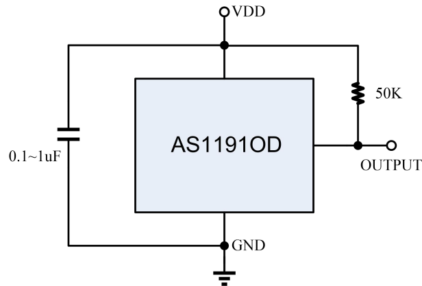
Figure 1, Typical Application Circuit of AS1191OD
